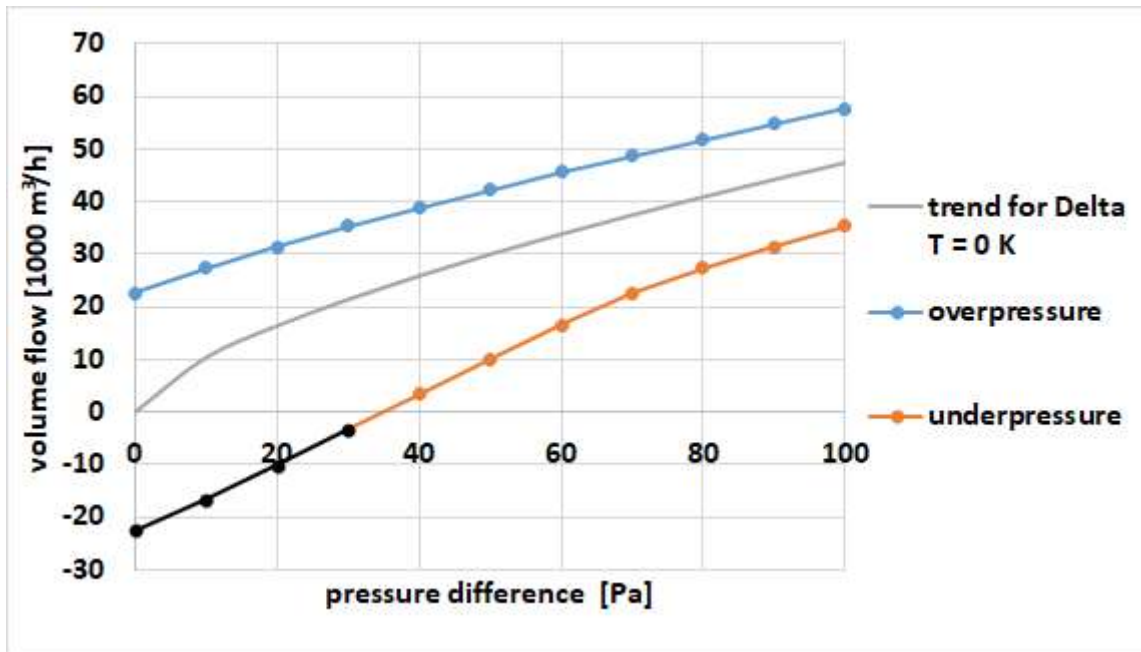
Figure 9: Measured volume flow and measured pressure difference if blower door installation and measurement take place at the ground floor. Since the zero pressure is already -35 Pa, the Blower Door would have to draw air into the building (black dots) to achieve lower negative pressures.
