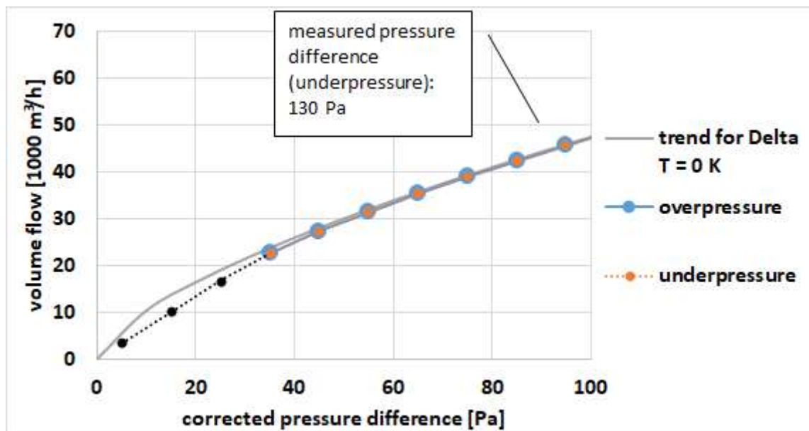
Figure 10: Measurement, as in Figure 6, the pressure difference is corrected by the zero pressure. If the corrected pressure difference is less than 35 Pa, the building is simultaneously under and over pressure (black dots).
